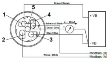
Connector plug A (M12 - A-coding) Connector plug B (M12 - A-coding)
