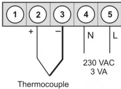
Type DAG-A3T0 with a supply of 230 VAC
