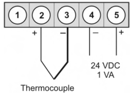
Type DAG-A3T3 with a supply of 24 VDC
